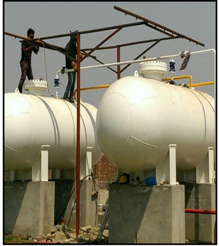
LPG Piping
